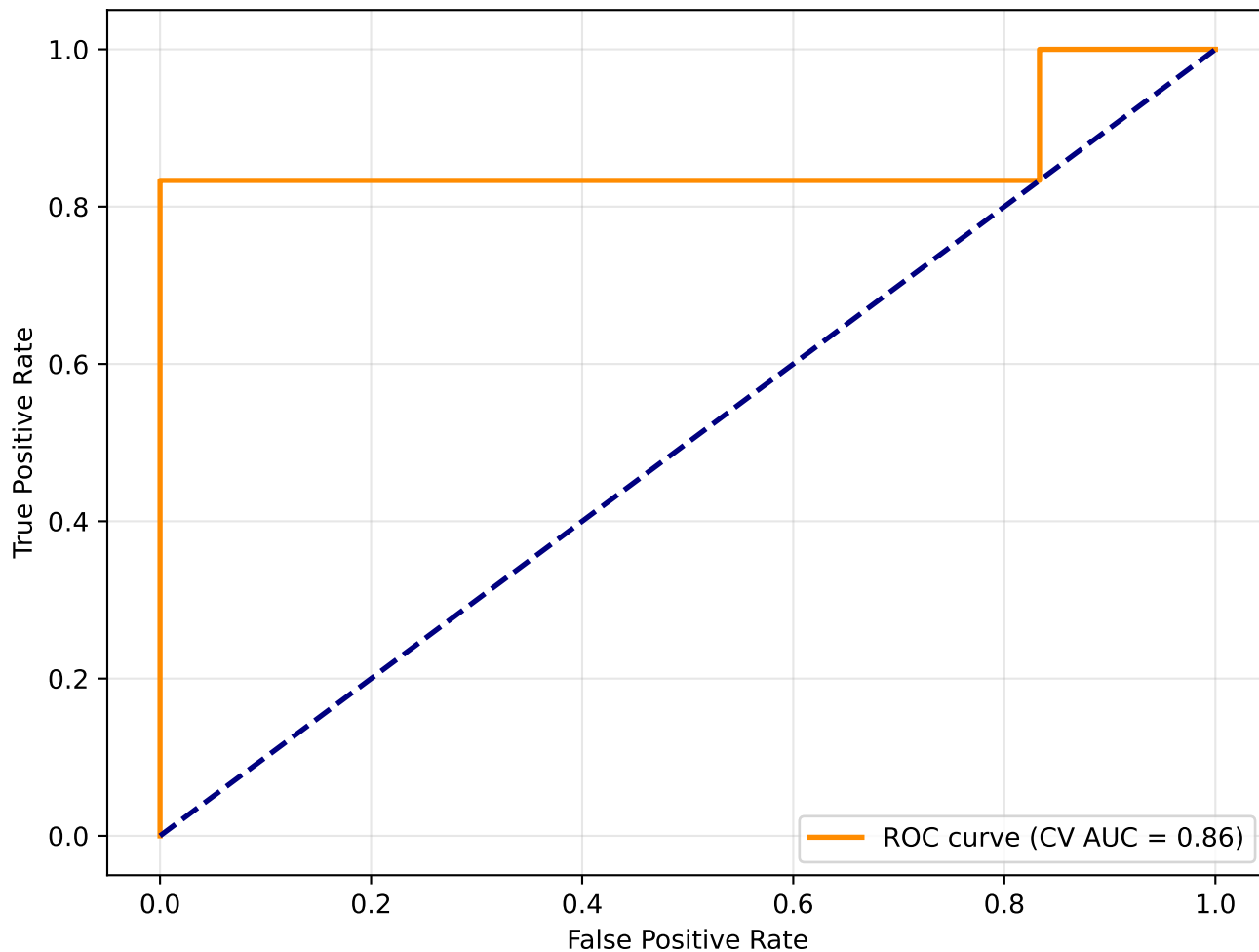
ROC Curve (Nested CV): T0 vs D17
