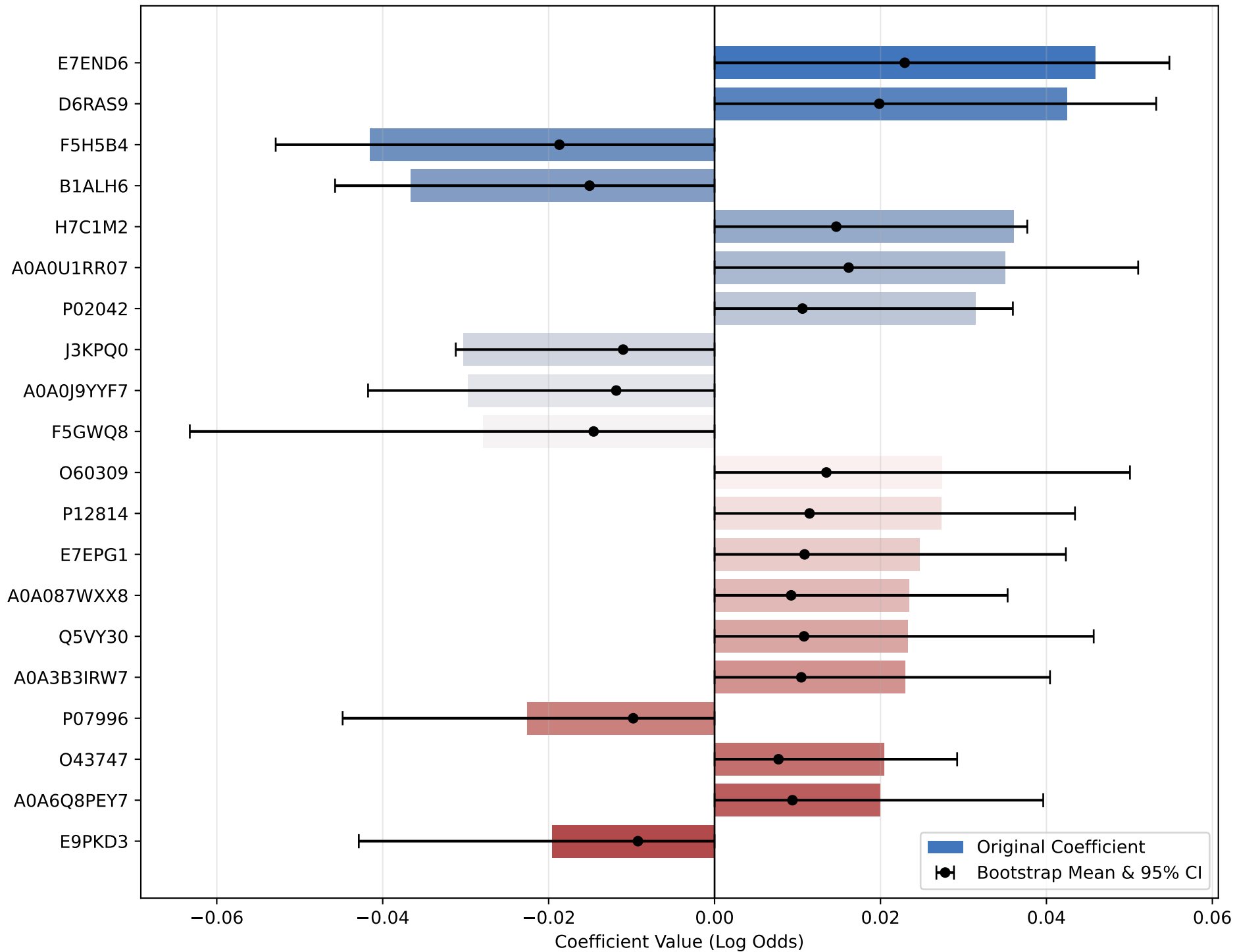
Top 20 Features (Bars = Original, Points/Lines = Bootstrap 95% CI)
